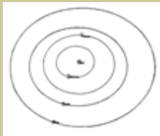
Comparative solar system diagram, 6 Sep 2003
