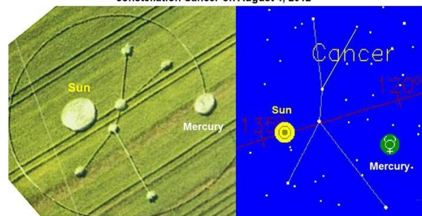
Comparison of "crop stars" from Santena, Italy with actual stars in the constellation Cancer on August 4, 2012
