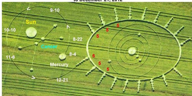
A general curve shows the schematic orbit of Mercury from August 4, 2012 to December 21, 2012
