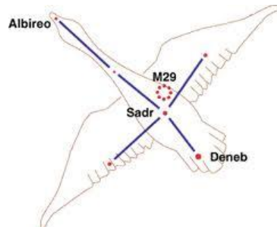
CYGNUS NEAR VEGA – VULTURE not far from Altair the eagle's feather
