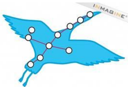
GRUS CRANE UNDER PISCES "SPUN IN CRANE" in the south
