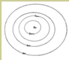
Comparative solar system diagram, 6 Sep 2003
